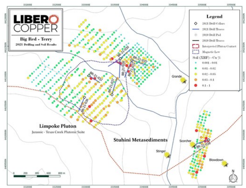
Figure 4: Plan map illustrating the distribution of drilling at the Terry target and the XRF Cu-in-soil results from the soil sampling programs. (CNW Group/Libero Copper & Gold Corporation.)
