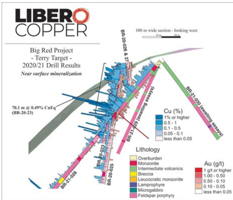
Figure 2: Zoomed cross-section of the upper portion of hole BR-21-028 and its relation to the RC holes drilled in 2020 and the positions of BR-21-029 and 030 which were drilled from the same pad as hole 28. (CNW Group/Libero Copper & Gold Corporation.)
